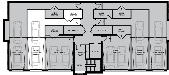
PARKING PLAN: 2-CAR TANDEM GARAGE
